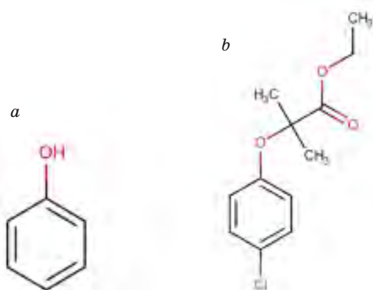
Fig. 1. Structure of Phenol (a) and Clofibrate (b)
