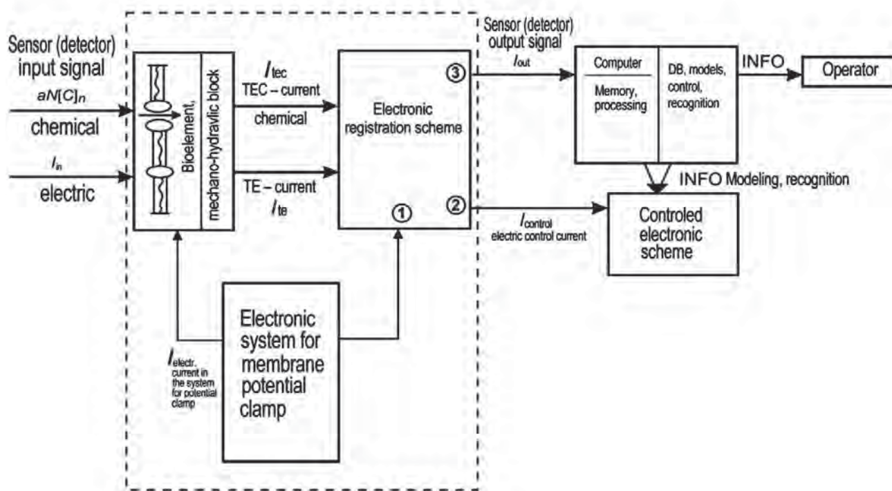
Fig. 2. Block diagram of the technical sensor system in the “EcoIS” (BTSM-3). This complex may be an element in the block “Measuring system” (Fig. 1): at the input of the system information comes in the form of electrical or chemical signals, at output — in form of electrical signals
