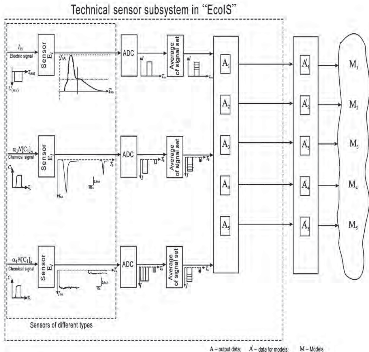
Fig. 3. From the electrical signals to the mathematical models: at the input of the BTS system with BF the information comes in the form of electrical or chemical signals, at output — in form of electrical signals. M — different mathematic models from the developed models family
