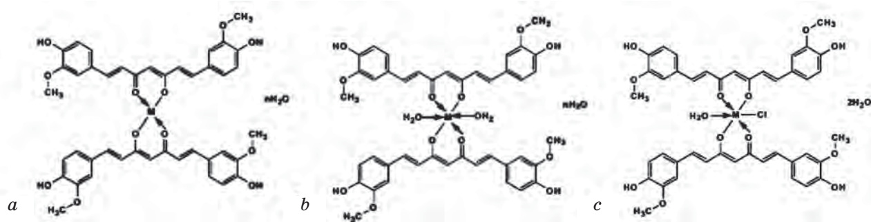
Fig. 11. Structure of curcumin complexes:
