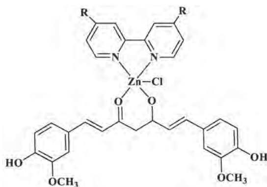
Fig. 13. Schematic representation of "curcumin — 4,4'bipyridyn" with \text{Zn}^{2+} complex [52, 54]
