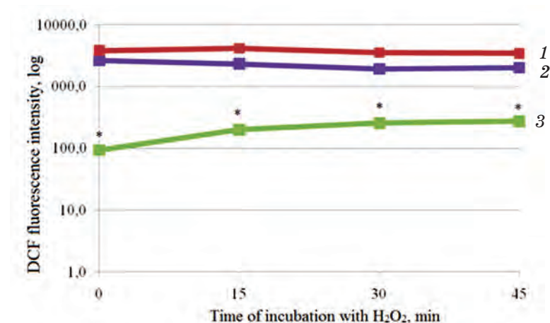
Fig. 8. DCF fluorescence intensity of lymphocytes (1), monocytes (2) and granulocytes (3) when adding exogenous H_2O_2 after cells isolation with dextran and freezing with 5% DMSO: * — P \leq 0.05 significant difference of I_{DCF} compared with monocytes and granulocytes
