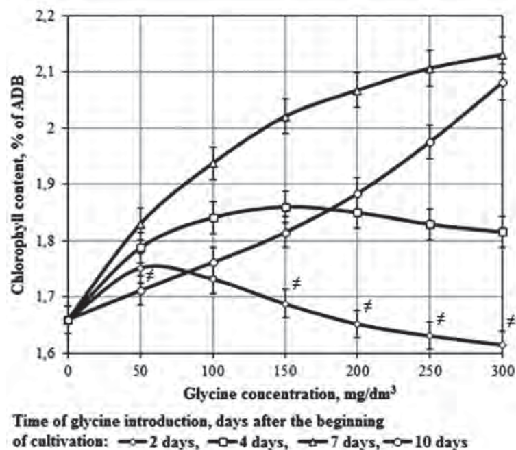
Fig. 4. Effect of glycine various concentrations on chlorophyll content
