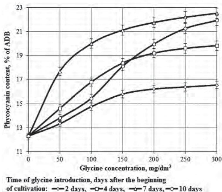
Fig. 2. Effect of glycine various concentrations on phycocyanin content
