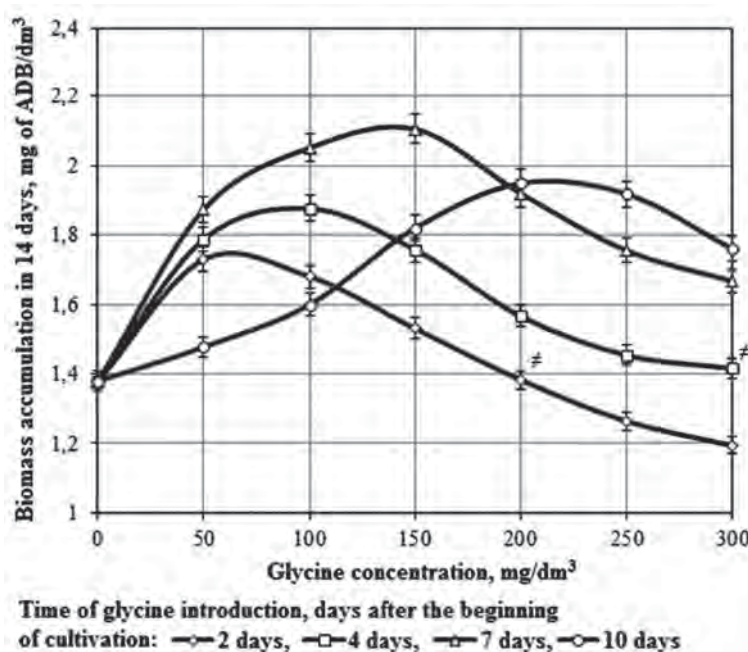
Fig. 1. Glycine influence on spirulina biomass accumulation depending on the time of its introduction: here and after results that do not have a statistically significant difference with the control (0% of glycine, P > 0.05 ) in the figures are indicated by \neq . Between nearby points there are insignificant distinctions that statistically not reliable
