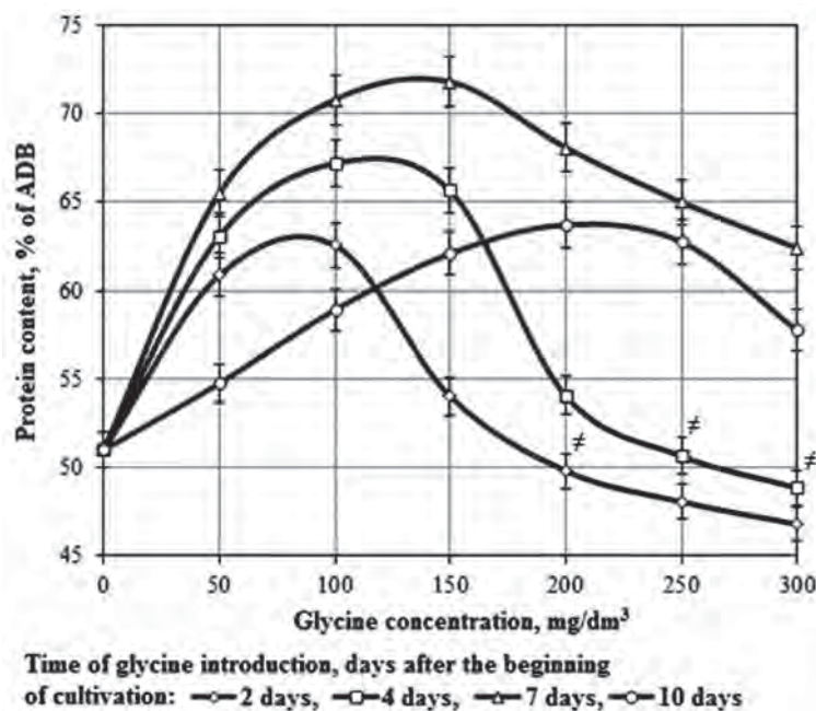
Fig. 3. Effect of glycine various concentrations on protein content
