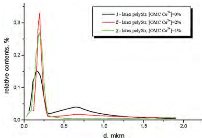
Fig. 5. Size distribution of luminescent polymeric nanoparticles:
