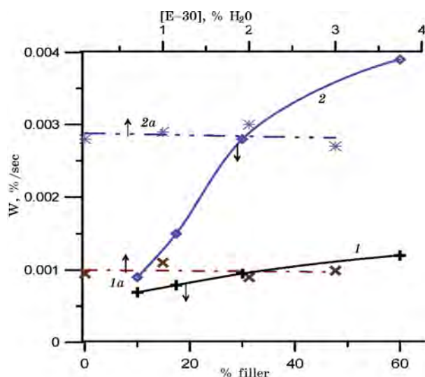
Fig. 15. Water dispersion polymerization rate of VEP-GMA*-St mixture vs. filler content (1, 2) and concentration of emulsifier E-30 (1a, 2a).
