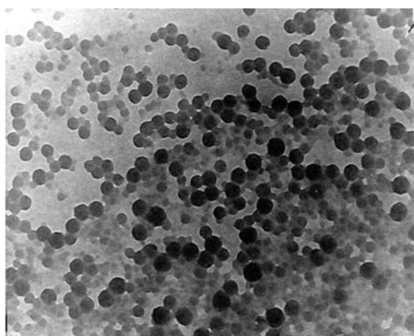
Fig. 6. TEM picture of polystyrene nanoparticles with functional shell containing coordinated \text{Ce}^{3+} cations:
